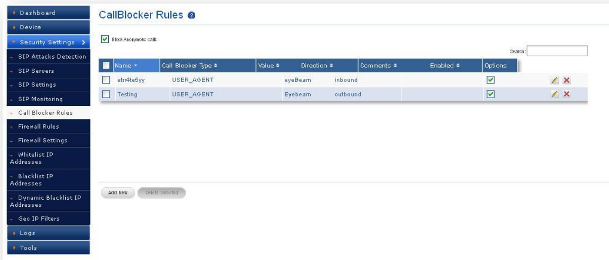
Figure 23: Call Blocker Rules
